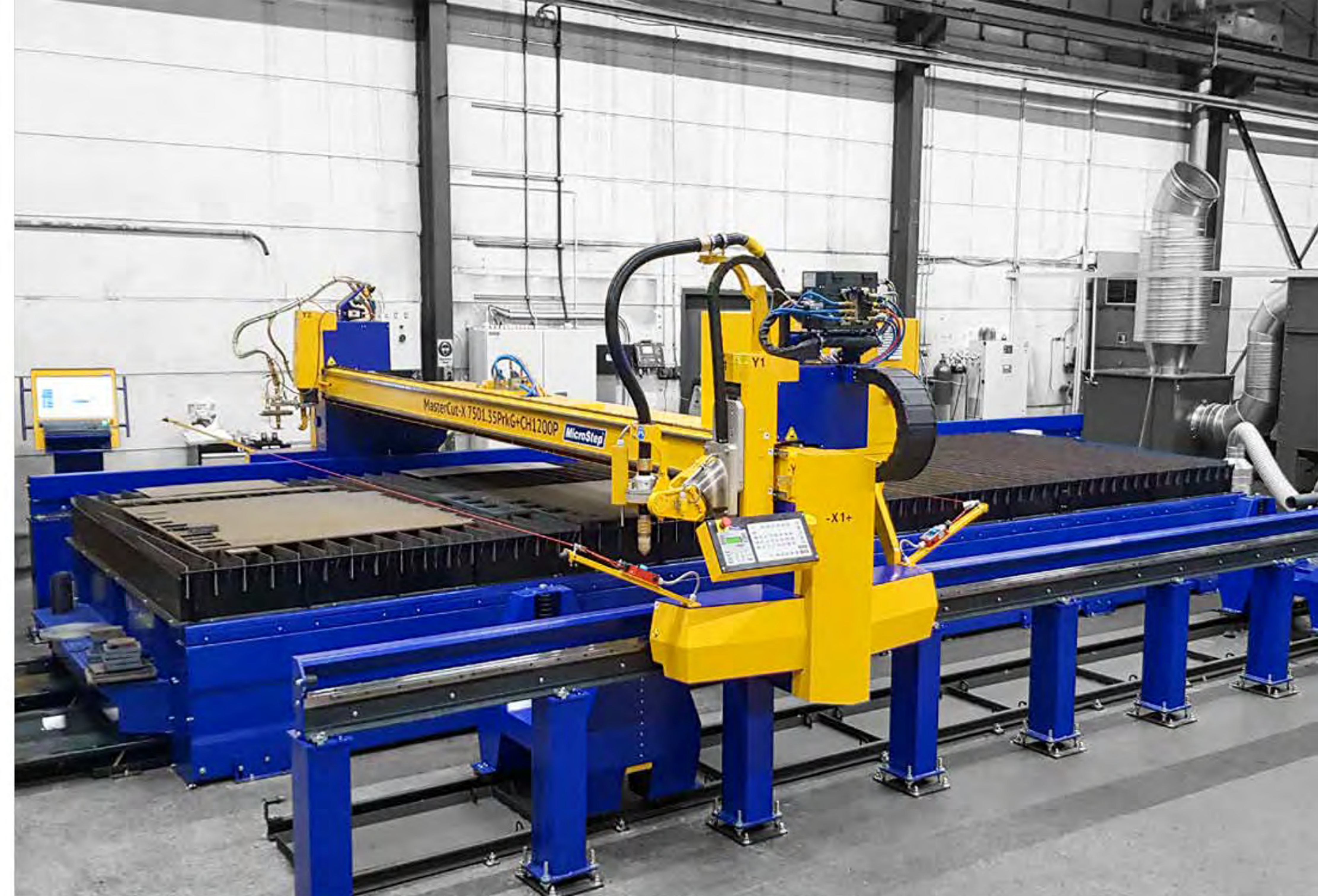
MasterCut with linear guidelines in the X-axis and a channel for pipe processing
