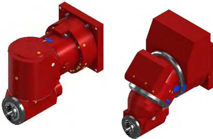
Indexing Milling Heads
